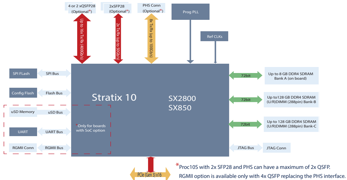
Proc10S System Block Diagram
